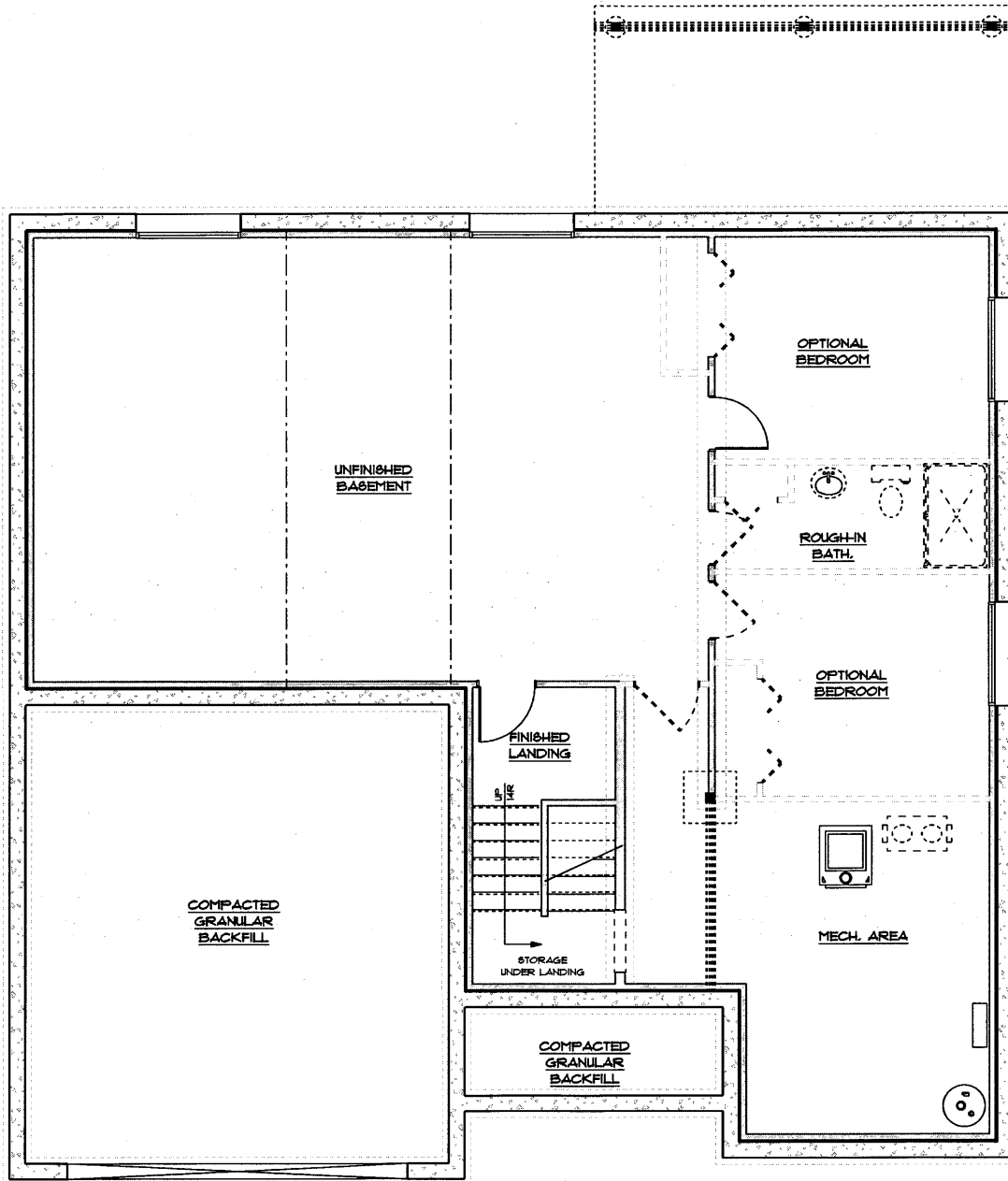
FOUNDATION PLAN E.I.O.E.
